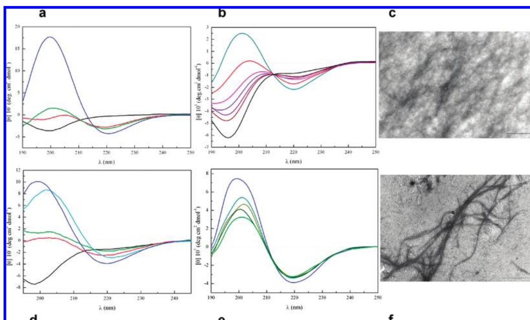
Figure 2. (a–c) Reversible self-assembly of KP. (a) CD spectra of 100 \mu M KP acquired at 20 ^{\circ} C using samples prepared from the stock solution kept at 4 ^{\circ} C for 1 h (black line), 3 days (red line), 1 month (light green line), and 6 months (blue line). (b) CD spectra of 100 \mu M KP prepared from the 1 month old stock solution as a function of time: (dark green line) 0 min, (red line) 20 min, (magenta line) 40 min, (violet line) 60 min, (dark purple line) 80 min, (maroon line) 100 min, and (black line) 330 min. (c) Electron micrograph of 1 mM KP prepared from the stock solution stored 24 months at 4 ^{\circ} C. Bar: 1 \mu m. (d–f) Catalytic effect of laminarin upon KP assembly and reversibility. (d) CD spectra of 100 \mu M KP prepared from the stock solution at different times: (black line) KP fresh solution, (red line) KP fresh solution + 500 \mu M laminarin, (light green line) KP 15 days old solution, (light blue line) KP 15 days old solution + 500 \mu M laminarin, (dark blue line) KP 5 months old solution. (e) CD spectra of 100 \mu M KP prepared from the 15 days old solution + 500 \mu M laminarin as a function of time: (dark blue line) 0 min, (dark green line) 60 min, (gold line) 120 min, (green line) 180 min, and (light green line) 240 min. (f) Electron micrograph of 1 mM KP from the stock solution soon after solubilization + 5 mM laminarin. Bar: 1 \mu m. All KP samples were prepared from a 2 mM stock aqueous solution stored as indicated above. CD measurements were carried out on a Jasco 715 spectropolarimeter (JASCO International Co. Ltd.) coupled to a Peltier PTC-348WI system for temperature control. CD far-UV spectra were recorded from 190 to 250 nm and averaged over four scans, using a 1 mm cell path. Following baseline correction, the measured ellipticity, \theta (mdeg), was converted to the molar mean residue ellipticity [\theta] ( \text{deg}\cdot\text{cm}^2\cdot\text{dmol}^{-1} ). For the electron microscopy studies, grids were prepared as previously described 18 and examined with a Philips EM 208S transmission electron microscope.
